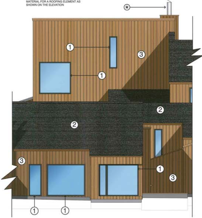
CLUSTER - PARTIAL ELEVATION
