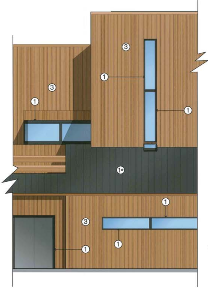
LODGE - PARTIAL ELEVATION
