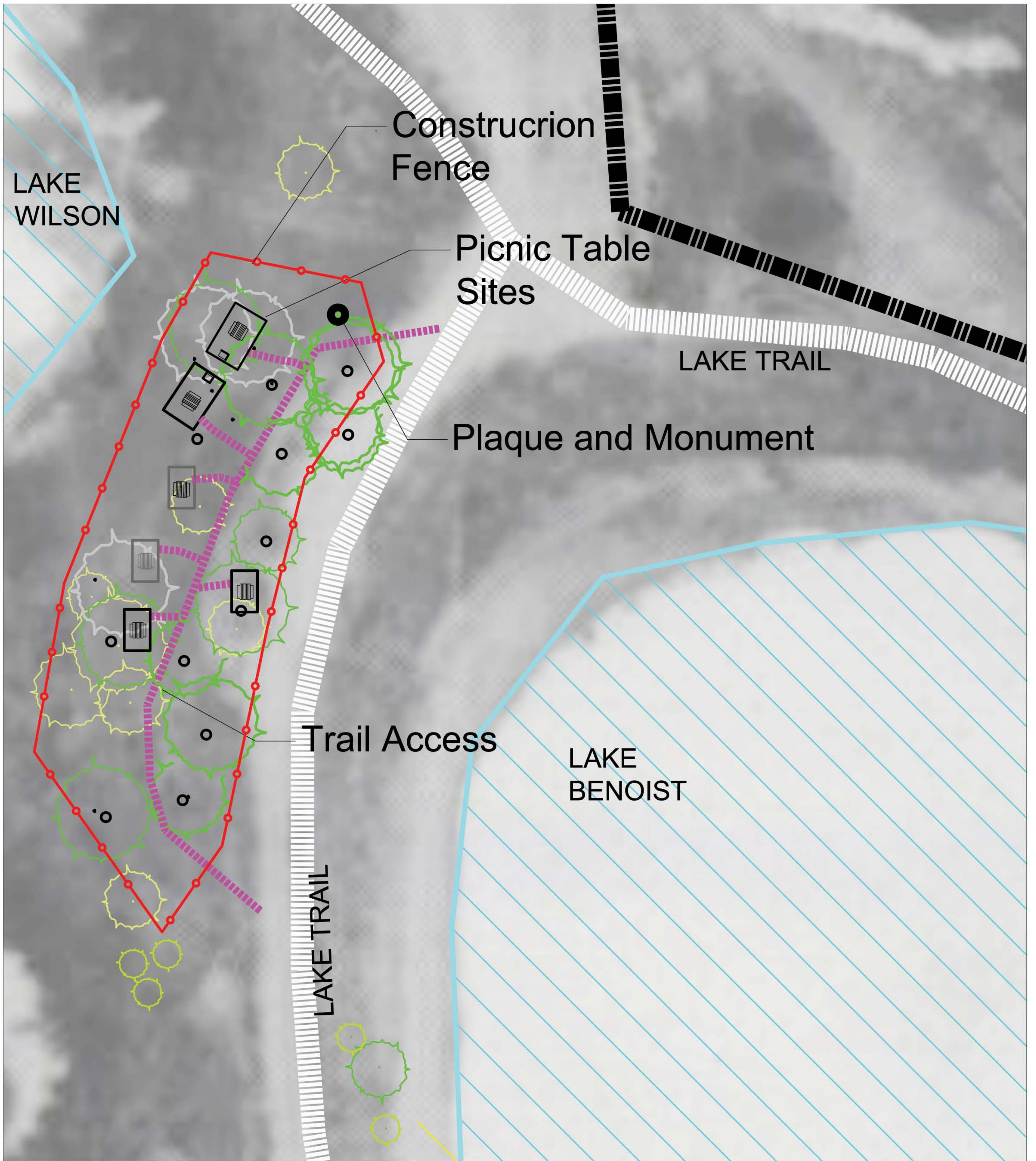
Riverfront Regional Park East Lake Picnic Area Site Plan
